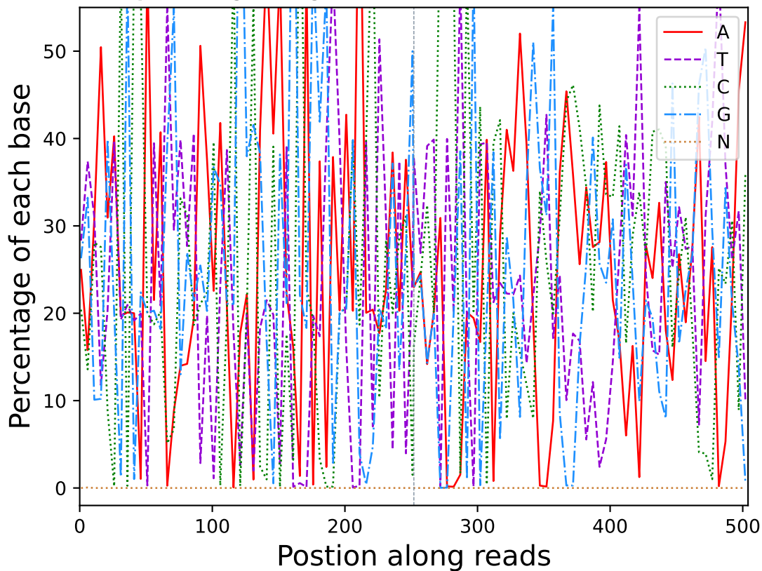
Base percentage along reads (R10528)
